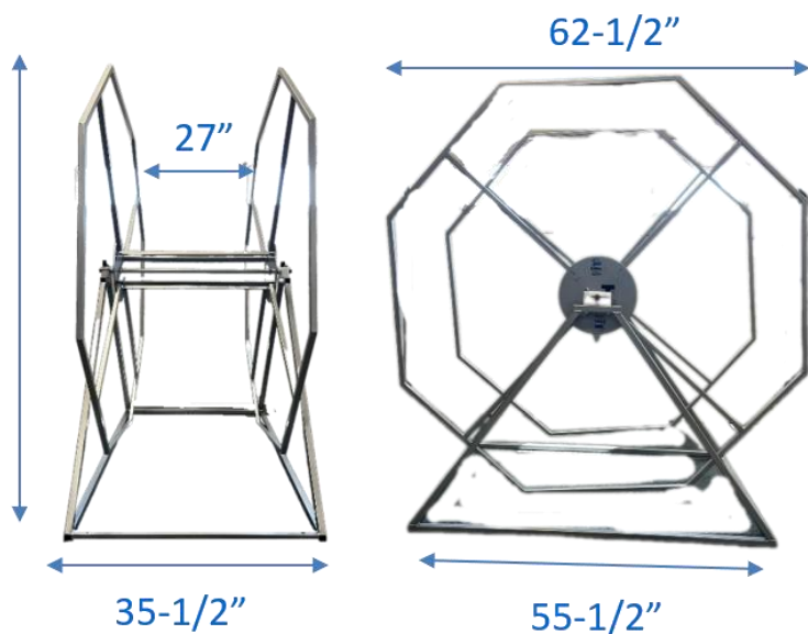
HR350 Dimensions
