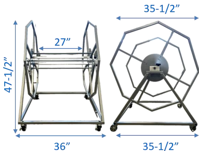
HR150 Dimensions
