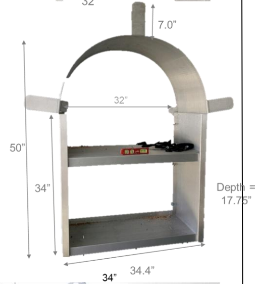
Description: Aluminum Hose Hood with two shelves
