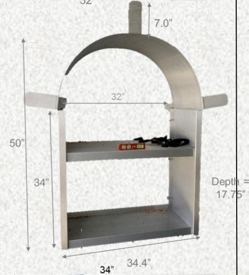
Description: Aluminum Hose Hood with two shelves
